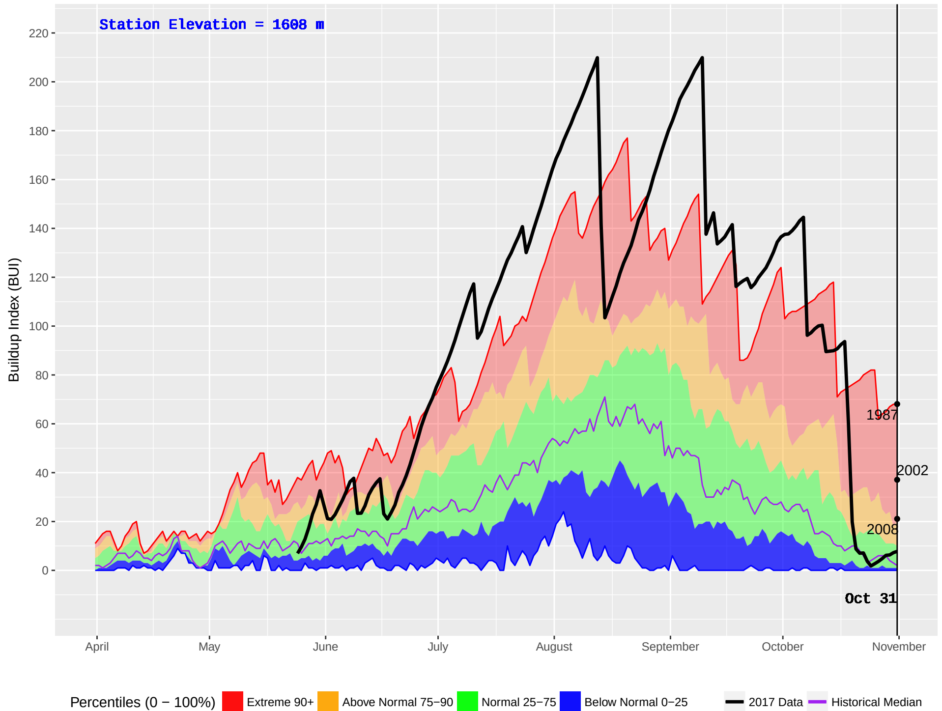
DEWAR CREEK (421) : Historical (1986–2016) and Current (2017) Noon Buildup Index (BUI)
